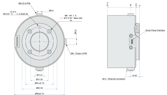
Tool flange for UR10g-1750
